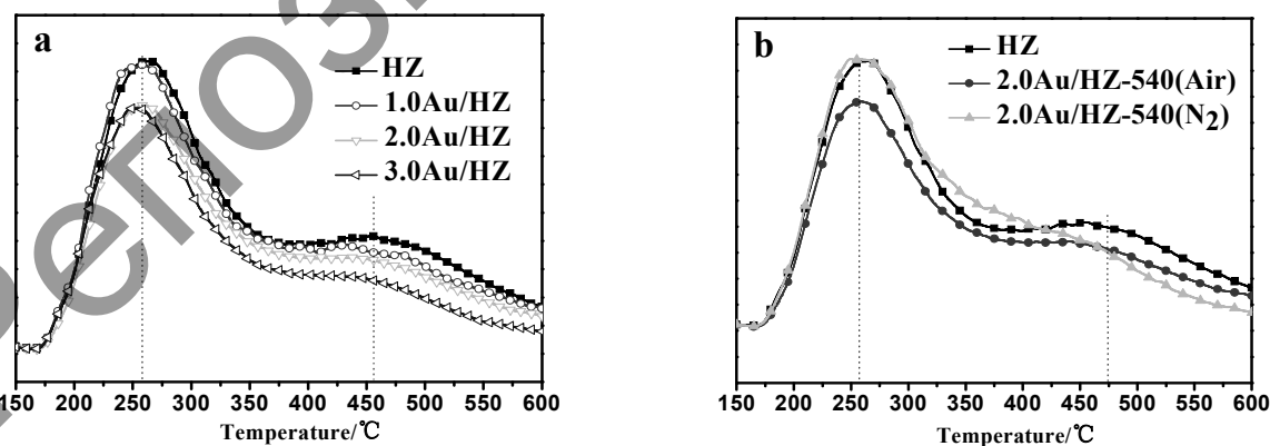
Figure 5. \text{NH}_3 -TPD profiles of Au/HZ catalysts calcined in air (a) and \text{N}_2 (b)
