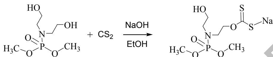
Figure 4. Scheme of dimethyl-bis(2-hydroxyethyl)phosphamidate reaction with carbon disulphide and sodium hydroxide
