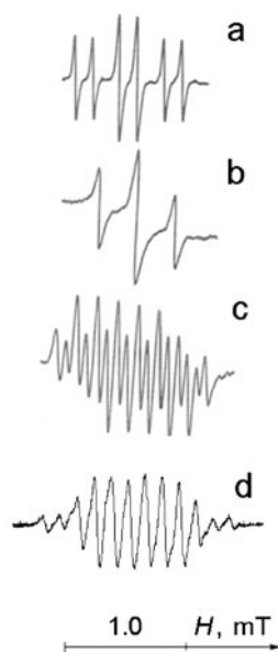
Fig. 4. EPR spectra of 3,6-di- tert -butyl-2-hydroxyphenoxy (a), ion pair of 3,6-di- tert -butyl- o -semiquinone with the cation of protonated polyethylenimine (PEI) (b), ion pair of I' chelated by polyethylenimine (PEI) molecules (c), and ion pair of I' chelated by hexamethylenediamine (HMDA) molecules (d) at room temperature.
