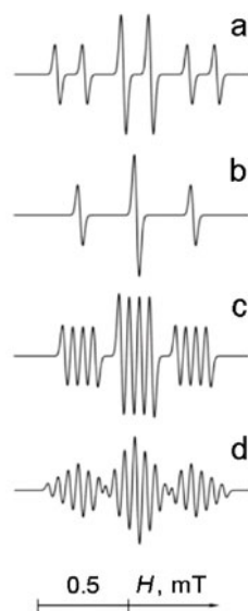
Fig. 2. EPR spectra of radical I and its derivatives at 293 K in toluene: a) hydroxyphenoxyl I, b) 3,6-di- tert -butyl- o -semiquinone radical-anion (I'), c) contact ion pair of I' with a lithium cation, d) dimer of the contact ion pair of I' with a lithium cation.
