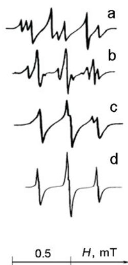
Fig. 1. Superposition of EPR spectra: a, b) radical I and ion pairs I' with the thebaine counterion at 253 K in toluene and at 263 K in tetrahydrofuran, respectively, c) contact and loose ions pairs of I' with triethylammonium cation at 263 K in tributyl phosphate, d) contact and loose ions pairs of I' in triethylamine.
