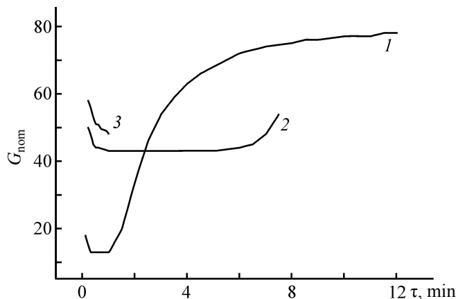
Fig. 1. Kinetic curves of (1) vulcanization, (2) scorching, and (3) viscosity of commercial vulcanized rubber for mines. ( G_{\text{nom}} ) Nominal shear modulus and ( \tau ) time; the same for Figs. 2–6.
