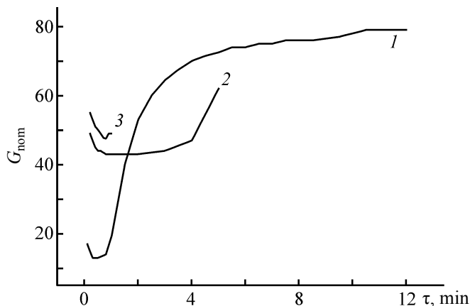
Fig. 4. Kinetic curves of (1) vulcanization, (2) scorching, and (3) viscosity of rubber compound prepared in accordance with formulation no. 3.
