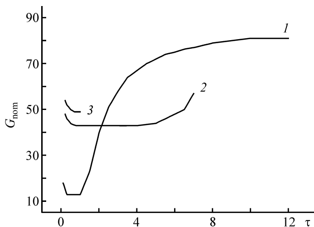
Fig. 6. Kinetic curves of (1) vulcanization, (2) scorching, and (3) viscosity of rubber stock prepared in accordance with formulation no. 5.
