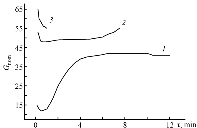
Fig. 3. Kinetic curves of (1) vulcanization, (2) scorching, and (3) viscosity of rubber stock prepared in accordance with formulation no. 2.
