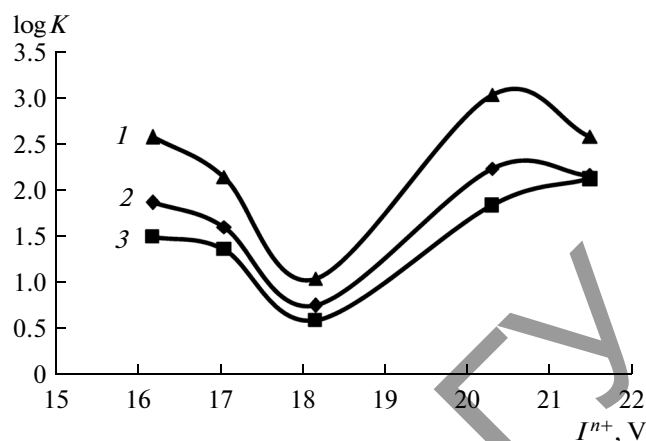
Fig. 2. Dependence of transition constant from an outer sphere complex to an inner sphere one on the ionization potential of metal ions. (1) (i-C 3 H 7 O) 2 PS 2 - ; (2) C 4 H 9 OCS 2 - ; and (3) (C 4 H 9 O) 2 PS 2 - .
