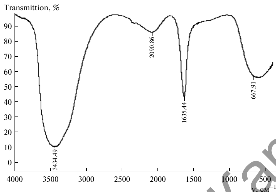
Fig. 1. IR spectrum of silver dibutyl dithiophosphate.
