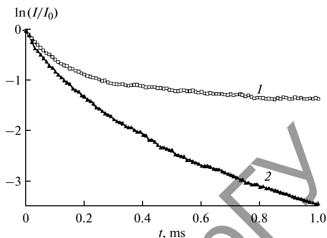
Fig. 2. Delayed fluorescence decay kinetics for the (1) PEPK + 1 wt % PD and (2) PEPK + 1 wt % MC films.
