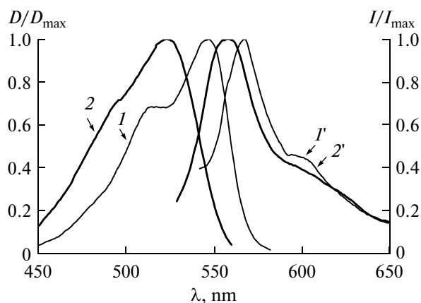
Fig. 1. (1, 2) Absorption and (1', 2') fluorescence spectra of the (1, 1') polymethine and (2, 2') merocyanine dyes in ethanol solutions. The concentration of the dyes was 10^{-5} mol L ^{-1} .
