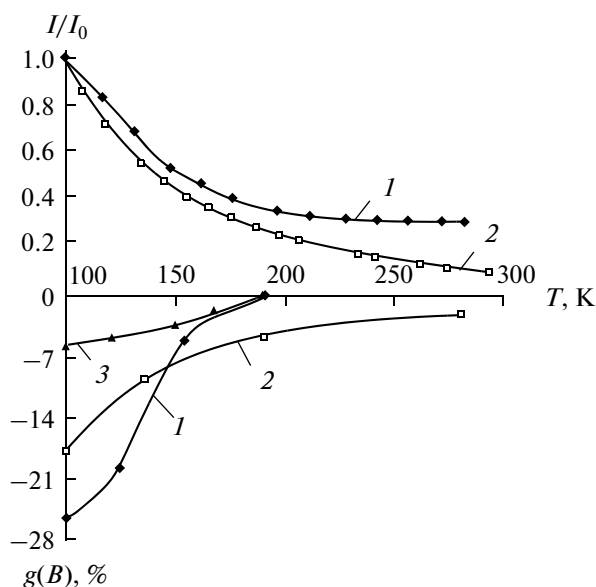
Fig. 5. Dependences of g(B) at B = 0.47 T and the RL intensity on T for the samples of (1) PEPK + 1 wt % PD, (2) PEPK + 1 wt % MC, and (3) KI-doped PEPK + 1 wt % PD.
