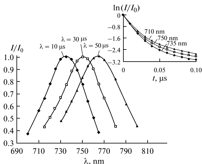
Fig. 3. Time-dependent phosphorescence spectra of the MC dye in PEPK. Inset: logarithmic dependences of the RL and phosphorescence intensities on the detection time.
