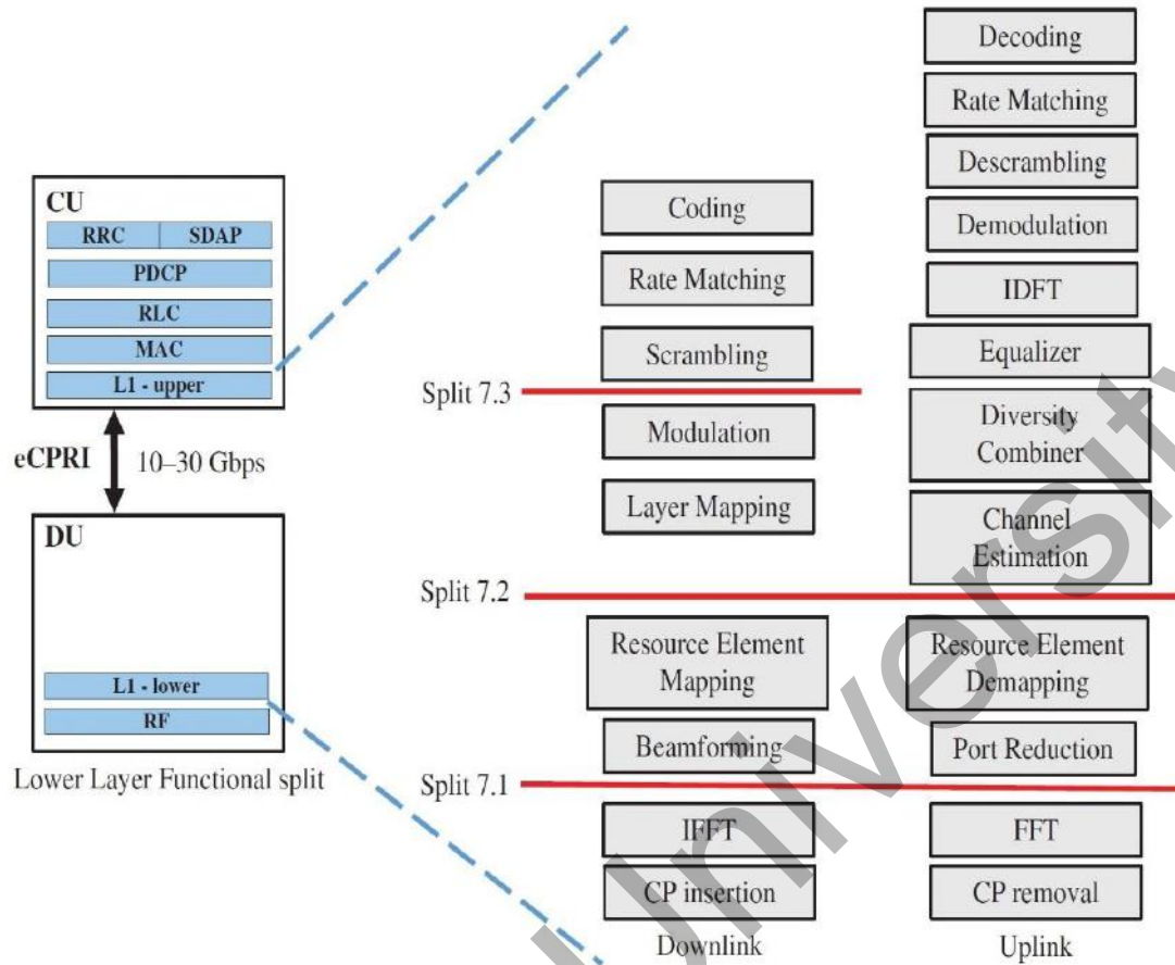
Fig.1. Options for Functional Partitioning 7 [19]
