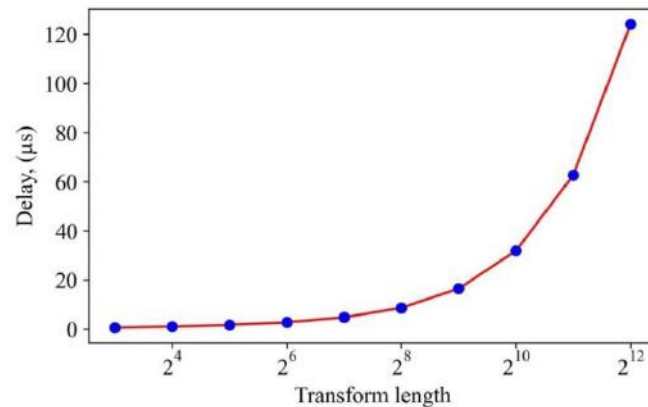
Fig.5. Dependence of Delay on FFT Module Size
