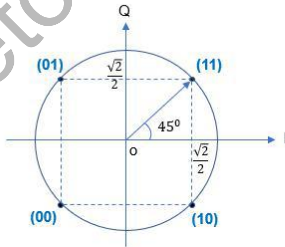
Fig.2. QPSK Constellations
